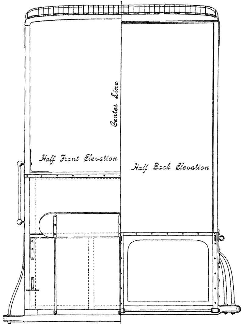
HALF FRONT AND HALF BACK ELEVATION OF FURNITURE WAGON DRAFT.
